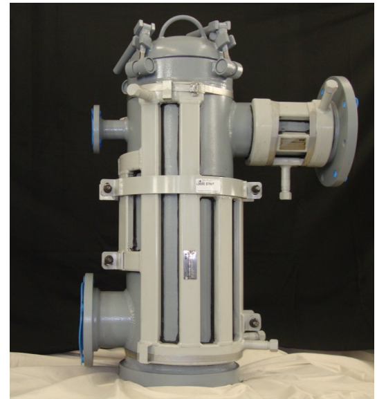
S x Seal™ 1000 sulfur sealing device, shown with ControTrace® steam tracing panels installed
